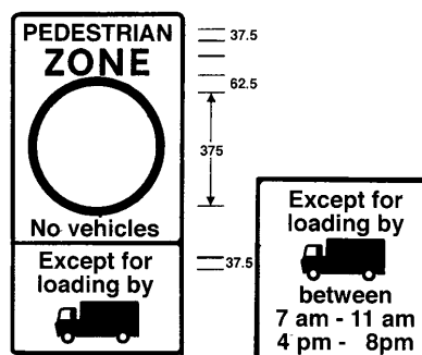
ENTRY TO PEDESTRIAN ZONE RESTRICTED (ALTERNATIVE TYPES)
